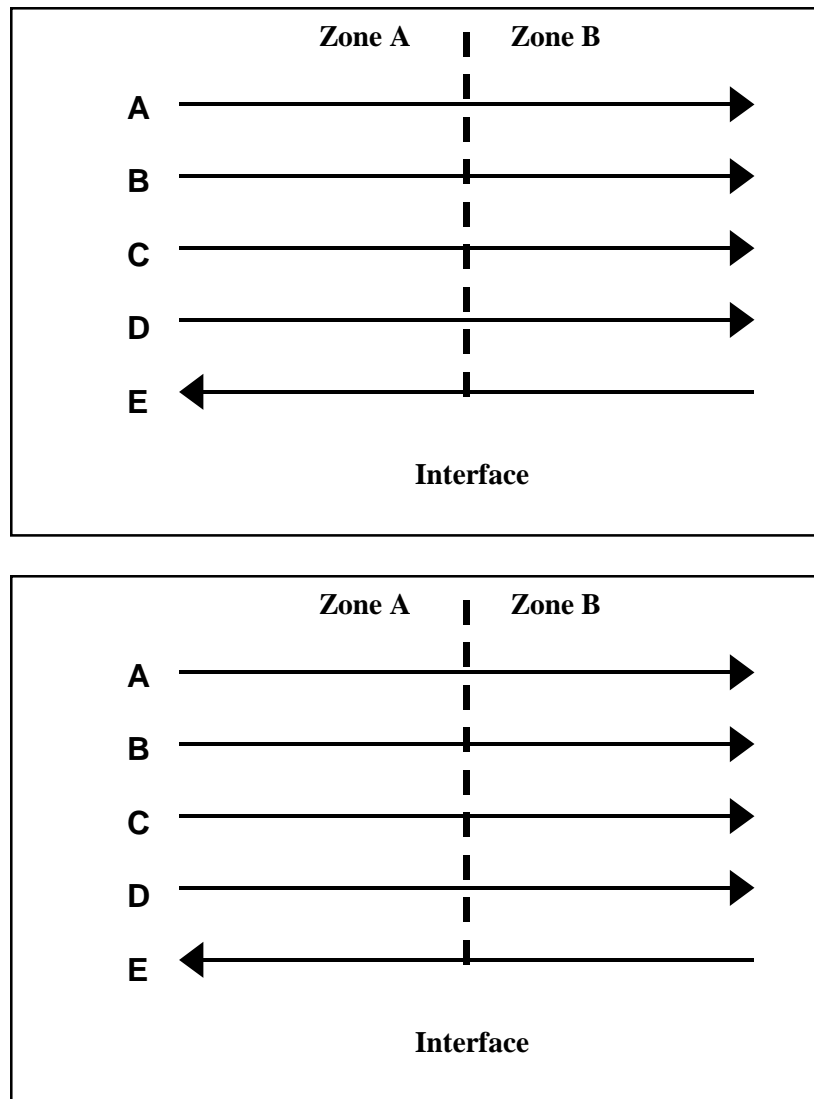
Figure 4-2: Transaction Example
